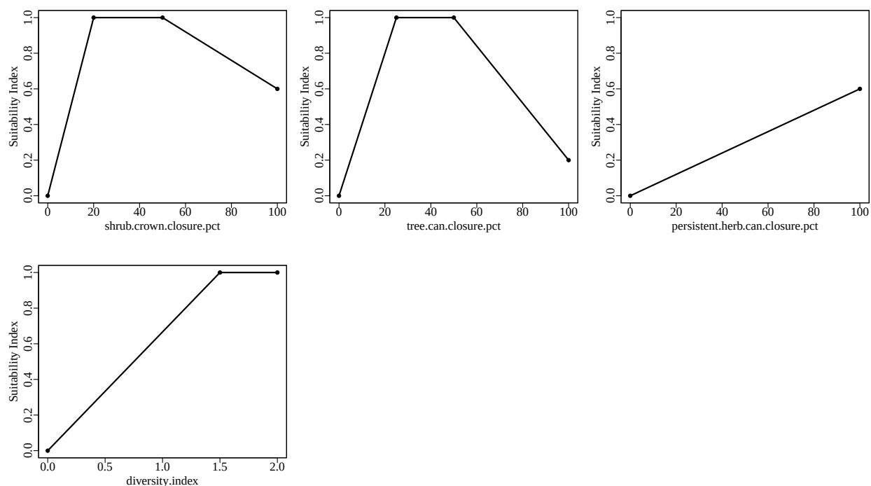
Figure 1. Suitability index graphs for variables included in the easterncotton model in ecorest .
